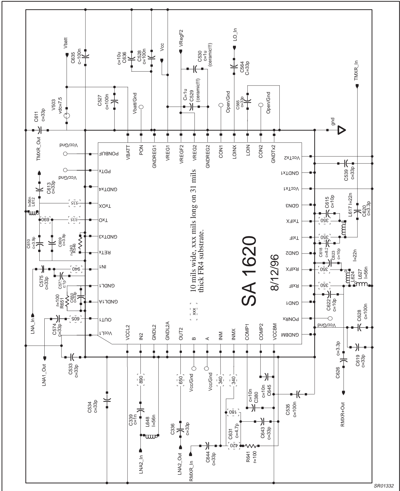
Figure 4. Application Circuit
